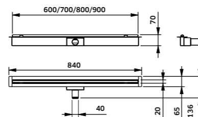
Canelete de Duche Horizontal Grelha SLIM 900mm
