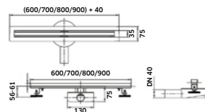
Canelete de Duche Horizontal Grelha SLIM 600mm
